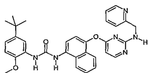
1-(5-tert-Butyl-2-methoxy-phenyl)-3-(4-{2-[(pyridin-2-ylmethyl)-amino]-pyrimidin-4-yloxy}-naphthalen-1-yl)-urea;
